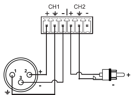
Balanced - XLR
